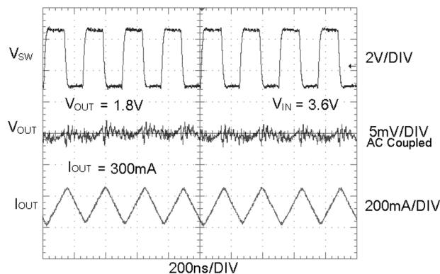
FIGURE 4. Typical PWM Operation
