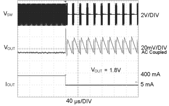
Load Transient Reponse ( V_{OUT} = 1.8V , PWM Mode to ECO Mode)
