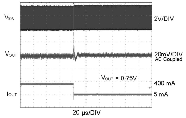
Load Transient Reponse ( V_{OUT} = 0.75V , FPWM Mode)
