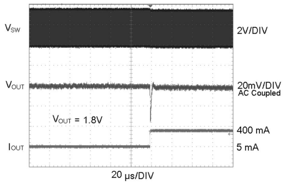
Load Transient Reponse ( V_{OUT} = 1.8V , FPWM Mode)
