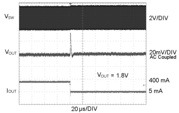
Load Transient Reponse ( V_{OUT} = 1.8V , FPWM Mode)
