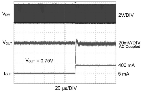
Load Transient Reponse ( V_{OUT} = 0.75V , FPWM Mode)
