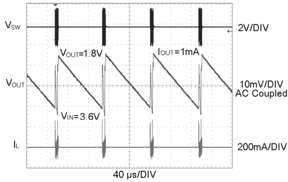
FIGURE 5. Typical ECO Operation
